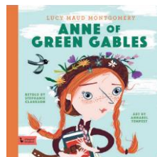
ANNE OF GREEN GABLES: A BabyLit® Storybook Stephanie Clarkson Illustrations by Annabel Tempest 9781423650713
